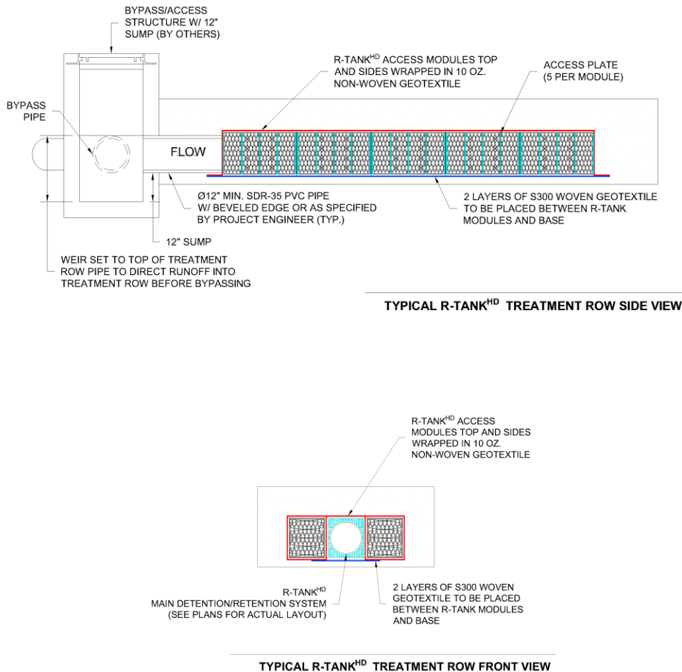
Figure 3 Typical R-Tank Treatment Row Section
