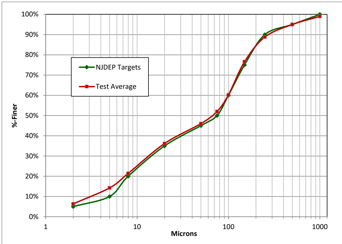
Figure 8 PSD Curves of 1-1000 micron Test Sediment
