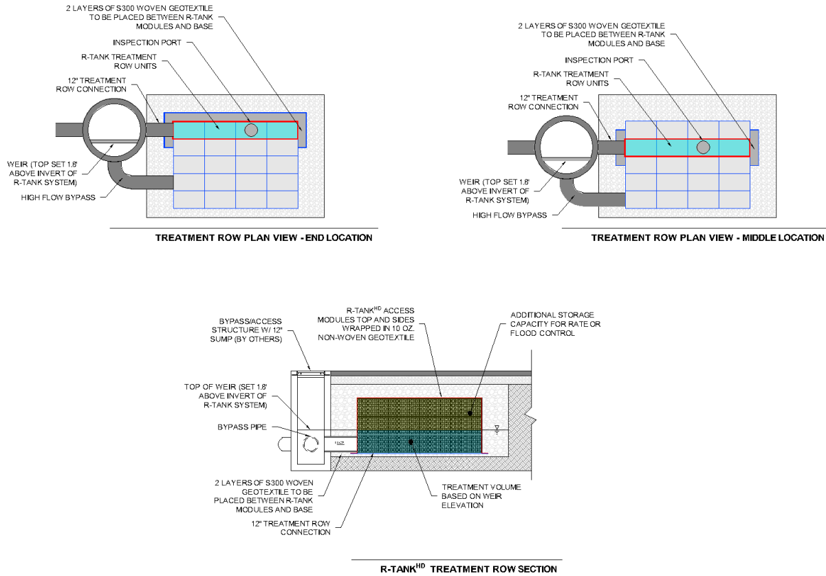
Figure 1 R-Tank Treatment Row Configurations
