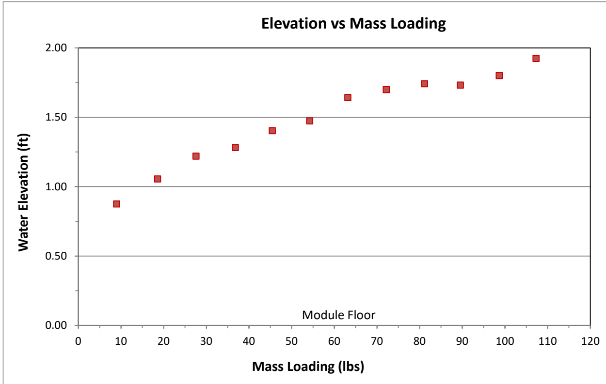
Figure 10 R-Tank Treatment Row End-of-Run Water Elevations
