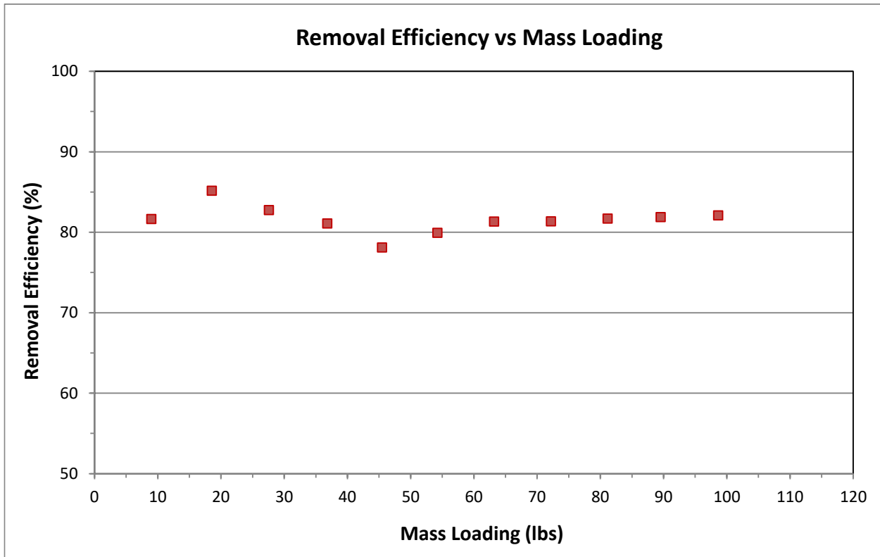
Figure 9 R-Tank Treatment Row Removal Efficiency vs Mass Loading
