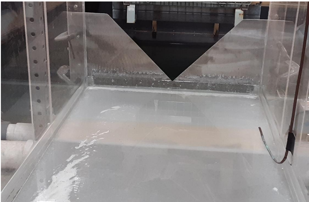
Figure 7 Effluent Channel V-notch Weir
