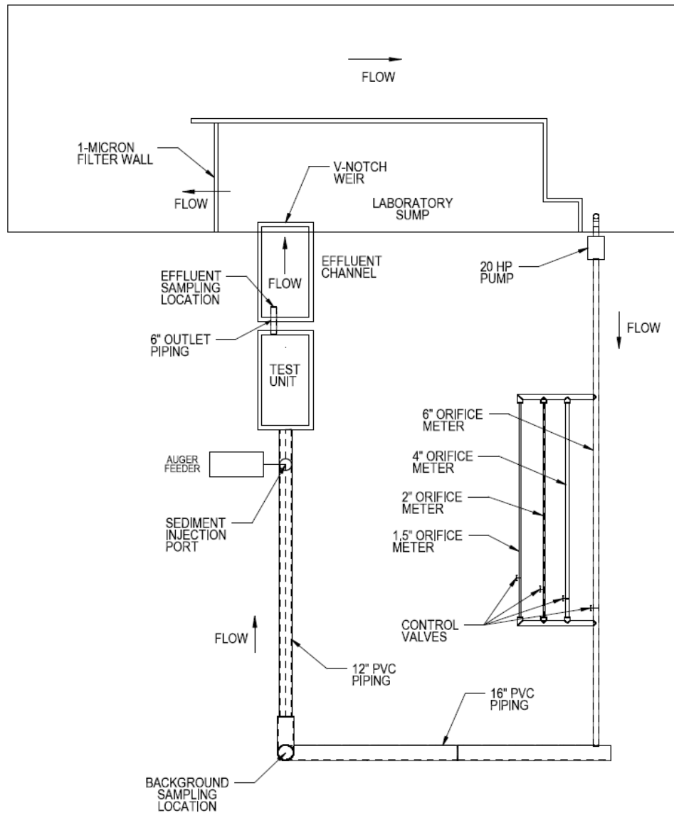
Figure 4 Alden's Stormwater Test Loop
