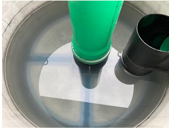
Figure 6 View from Top into a Concrete Manhole Version (HSVF-1000)
