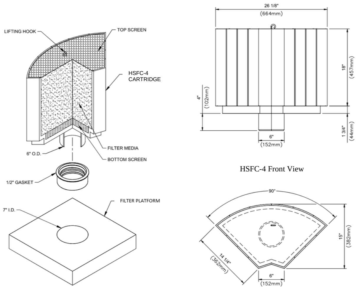
Figure 2 Hydrosystem® Filter Cartridge HSFC-4 Detail
